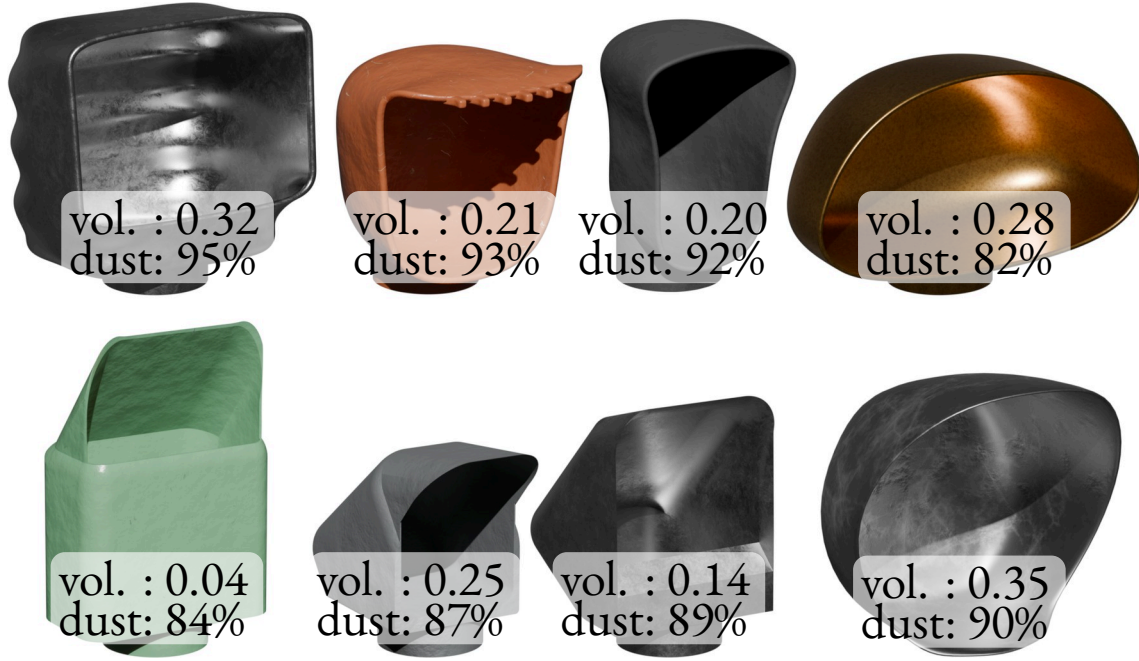
Figure 6.15 – The performance of the VISUAL agent across the held-out set of novel tool geometries. The results show significant performance variation based on tool design, highlighting the potential for data-driven hardware optimization.
