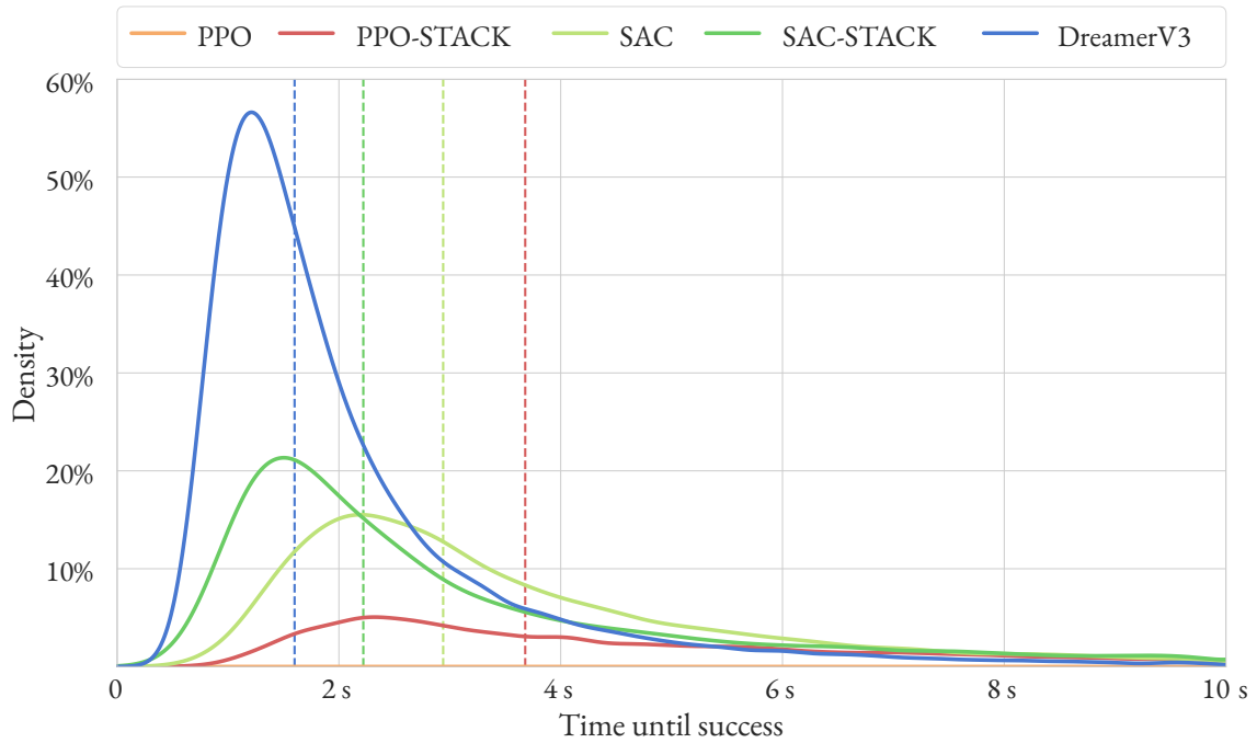
Figure 5.4 – Time until successful completion for the peg-in-hole assembly task. DreamerV3 demonstrates the fastest completion times, followed by the SAC variants.
