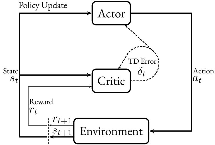
Figure 2.5 – The interaction loop of actor-critic RL. The actor (policy) selects an action, and the critic (value function) evaluates the quality of that action. The critic’s feedback is then used to update the actor, guiding it toward more rewarding behaviors.
