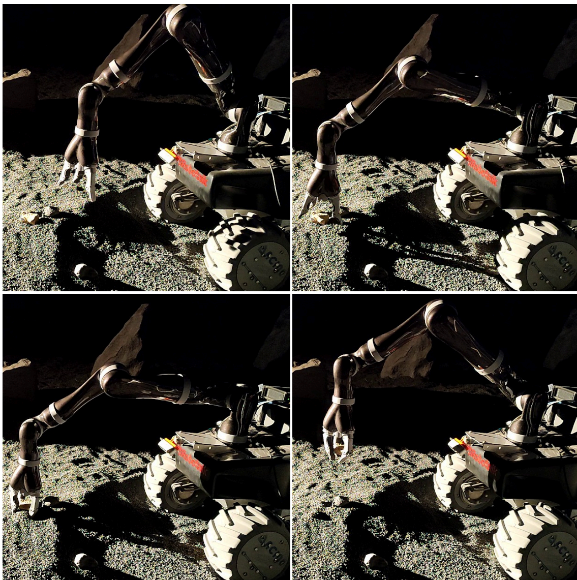
Figure 3.9 – A successful real-world grasp sequence.
