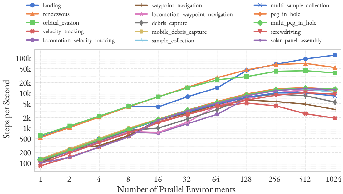
Figure 4.5 – The aggregate throughput of SRB tasks.
