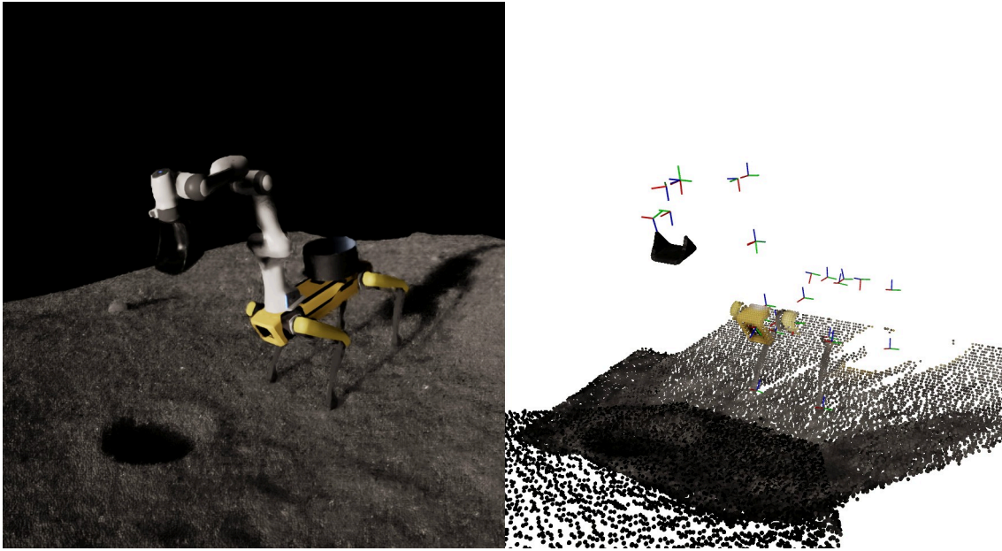
Figure 4.9 – An example of the ROS 2 interface showing the RViz2 visualization of the state and visual observations for a mobile manipulator inside an SRB simulation.
