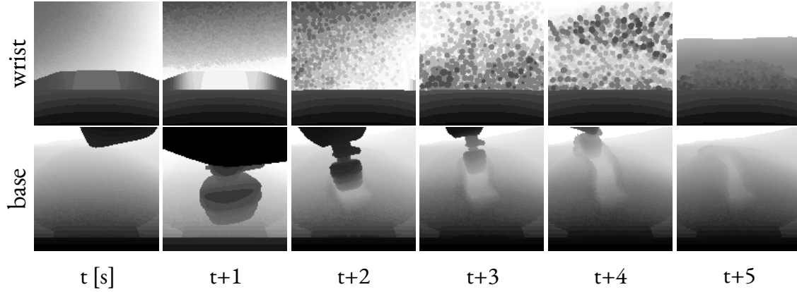
Figure 6.13 – Visual feedback provided to the VISUAL agent from two camera views over the course of a single excavation episode. The depth maps provide rich and real-time information about the robot workspace.
