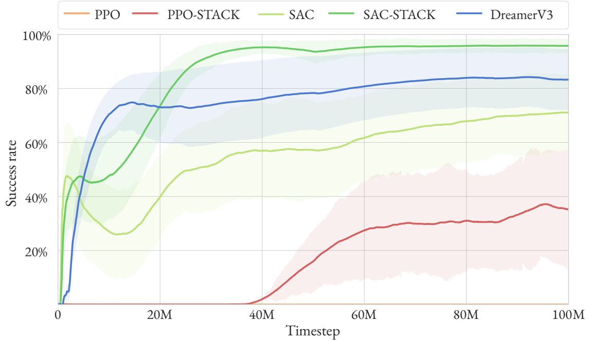
Figure 5.3 – Learning curves for the peg-in-hole assembly task from Publication II , comparing model-free (PPO, SAC) and model-based (DreamerV3) algorithms.
