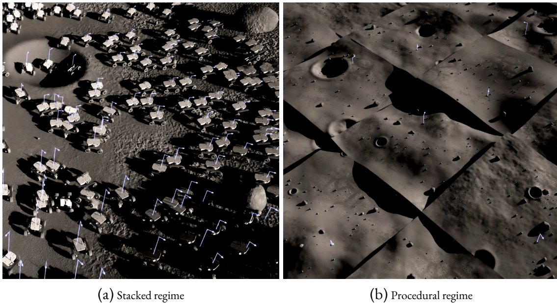
Figure 6.2 – Parallel simulation regimes of SRB. In the stacked regime, all agents share a single static terrain, risking overfitting. In the procedural regime, each parallel environment instance is exposed to a unique terrain to foster generalization.
