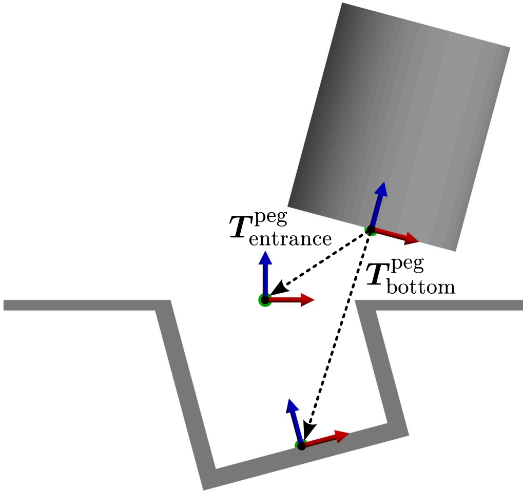
Figure 5.2 – The observation space of the peg-in-hole agents is defined by the T_{\text{entrance}}^{\text{peg}} and T_{\text{bottom}}^{\text{peg}} transformations that capture the kinematic state of the assembly.
