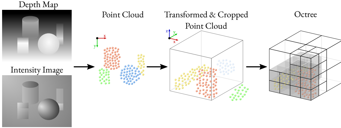
Figure 3.4 – The process of creating an octree-based scene representation. A raw point cloud is generated from sensor data. This point cloud is then transformed into the robot base coordinate frame and cropped to a fixed volume. Finally, it is voxelized into an efficient octree data structure, which serves as the primary visual input for the learning agent.
