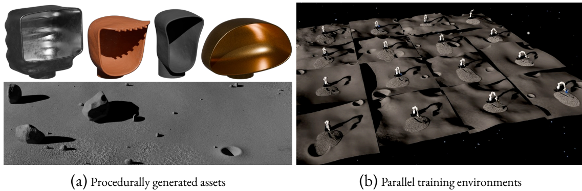
Figure 6.11 – The procedural paradigm for the excavation task, where PCG pipelines generate diverse terrains and tools that are then used to populate parallel environment instances.
