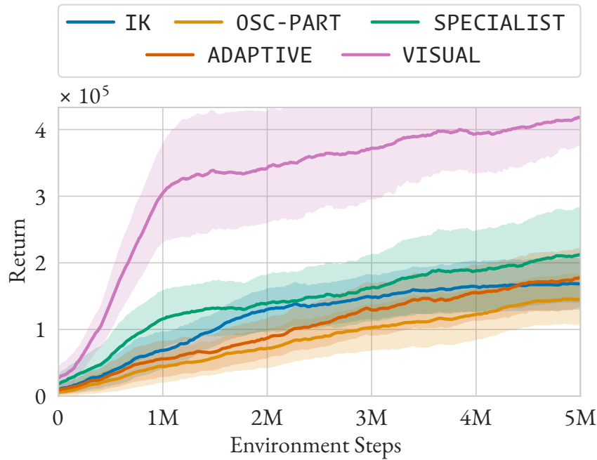
Figure 6.14 – Learning curves for the excavation task, where the VISUAL agent, trained with vision on diverse PCG tools, achieves the highest final performance.
