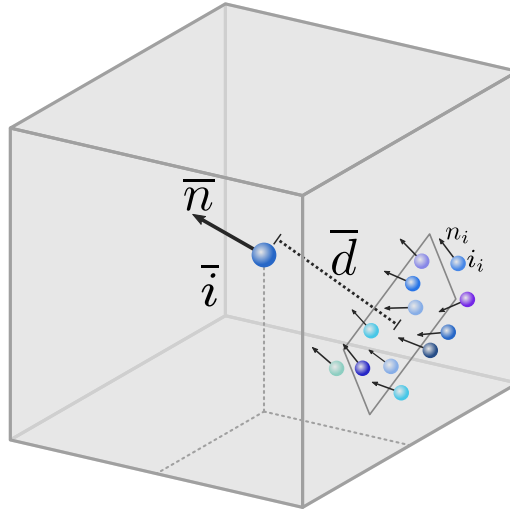
Figure 3.5 – A representation of the features stored within a single leaf octant of the octree. All points from the source point cloud that fall within the volume of a cell are used to compute the average unit normal vector \bar{n} , the average distance to the cell center \bar{d} , and the average intensity \bar{i} .
