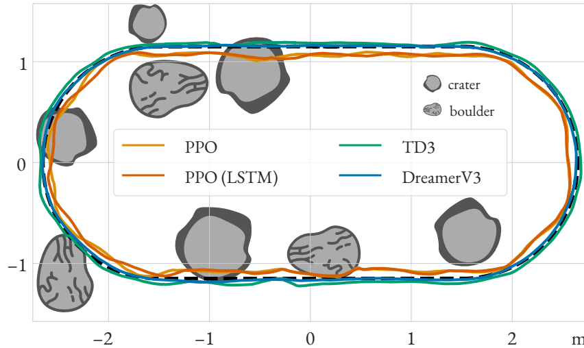
Figure 6.6 – Real-world trajectories of the physical rover following a capsule-shaped path, controlled by policies trained with different RL algorithms.
