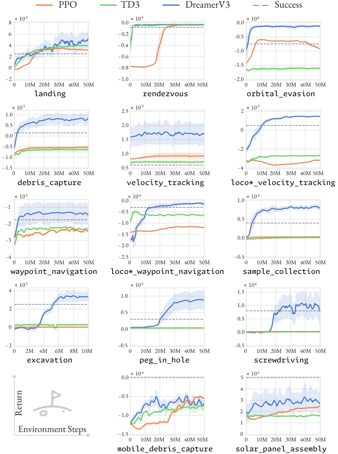
Figure 5.5 – RL baselines across SRB tasks from Publication VII. The results compare the performance of PPO, TD3, and DreamerV3 agents. DreamerV3 achieves the highest performance on most tasks.
