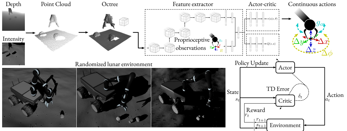
Figure 3.3 – An overview of the end-to-end learning approach. Visual data from a stereo camera is converted into a 3D octree representation. This, along with proprioceptive data, is fed into a shared feature extractor. The resulting features are then used by separate actor and critic networks to produce continuous task-space actions for the robot EE.
