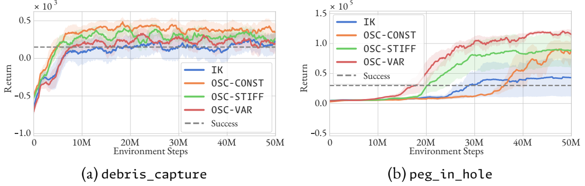
Figure 5.8 – Learning curves comparing different control strategies on the debris_capture and peg_in_hole tasks. The adaptive OSC variants (OSC-STIFF and OSC-VAR) exhibit task-dependent convergence and final returns relative to the rigid IK approach.
