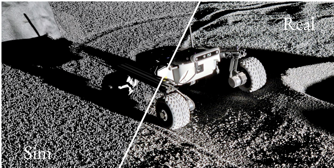
Figure 6.1 – The conceptual parallel for the adaptive traversal case study from Publication V , where agents are trained in SRB to track dynamic waypoints across diverse, procedurally generated scenarios. The generalization learned from this experience enables the acquired policies to transfer to a physical rover operating on granular media in a lunar-analog facility.
