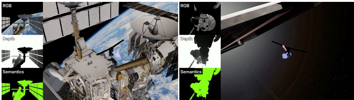
Figure 4.10 – Orbital inspection scenario of SRB providing synchronized RGB, depth, and segmentation streams from an onboard camera maneuvered around the ISS and Gateway.
