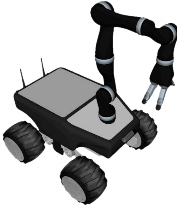
Figure 3.2 – The Summit XL-GEN mobile manipulator, with a 7-DoF Kinova Gen2 robotic arm and a stereo camera, which was used in both the simulation and the physical experiments.
