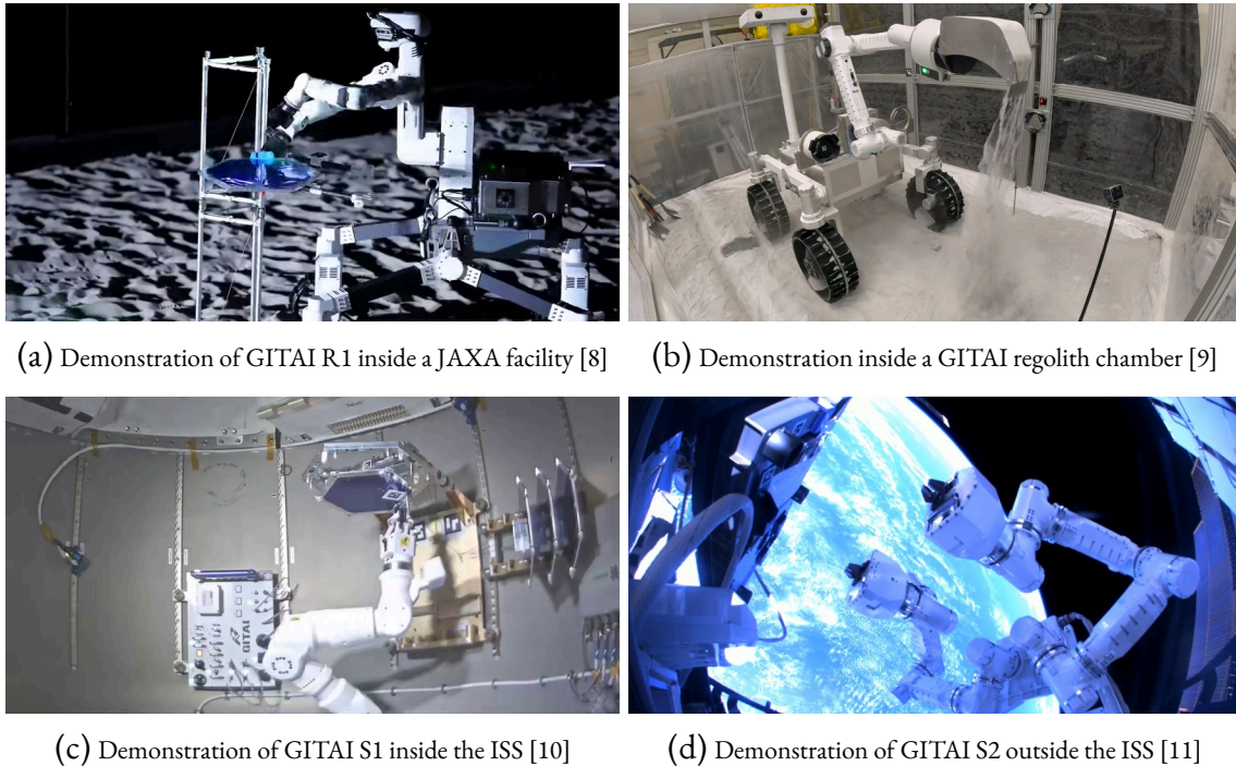
Figure 1.2 – Technology demonstrations of GITAI for in-space operations that illustrate the manipulation skills required for both planetary and orbital domains.
