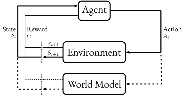
Figure 2.6 – The interaction loop of MBRL. The agent learns a world model from real-world interactions. It then uses this model for planning or to generate imagined trajectories, which are used to efficiently update the policy without requiring further real-world interaction.
