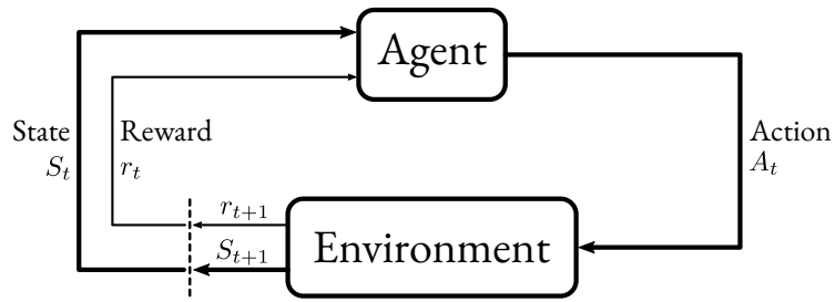
Figure 2.4 – The fundamental interaction loop of RL. The agent takes an action in the environment, which transitions to a new state and emits a reward. The agent uses this information to update its policy and inform future actions.
