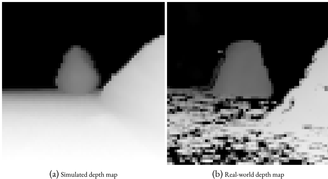
Figure 6.9 – Comparison of simulated and real-world depth views. The simulated map is clean, while the real-world image suffers from significant noise and signal dropout due to the properties of the basalt gravel.
