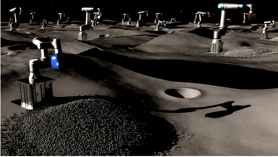
Figure 4.4 – The parallel architecture of SRB in action during the training of the excavation task. Each of the 64 environment instances features a unique PCG terrain and a distinct particle physics system for simulating the granular regolith as discrete particles.
