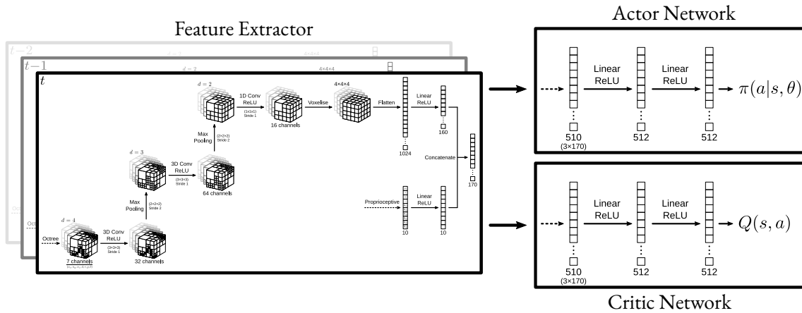
Figure 3.6 – The network architecture for octree observations. The encoder uses 3D convolutions followed by max pooling and pointwise convolution. Extracted visual features are flattened, combined with proprioception, stacked, and then used by the actor-critic networks.
