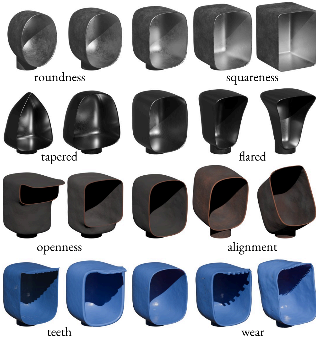
Figure 6.12 – A grid of PCG excavation tool geometries from Publication VI.
