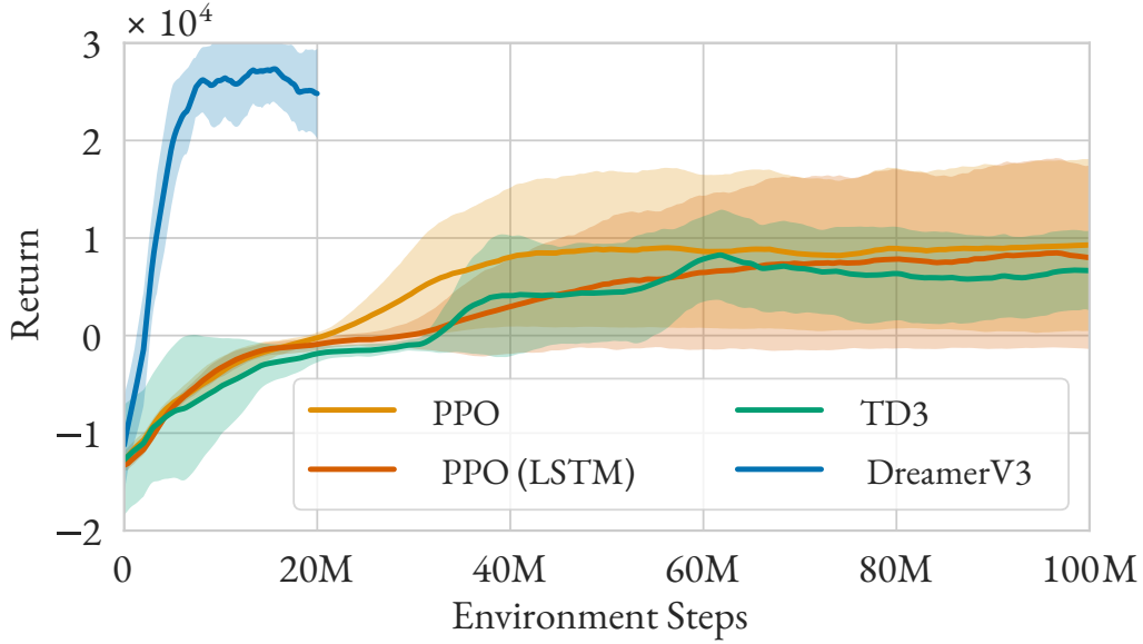
Figure 6.5 – Learning curves of the evaluated RL algorithms from Publication V . The results are averaged over five random seeds, with shaded regions representing the standard deviation. DreamerV3 demonstrates superior sample efficiency and achieves a higher final return.
