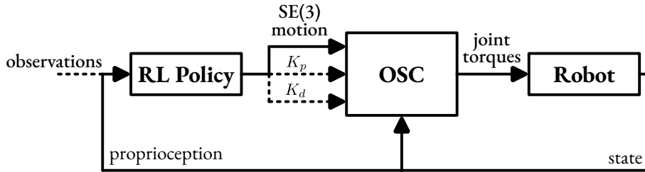
Figure 5.9 – Conceptual illustration of adaptive compliance through OSC. The RL agent learns to dynamically modulate the EE’s stiffness and damping parameters in addition to its SE(3) motion commands, enabling it to adapt its physical interaction strategy in real time.
