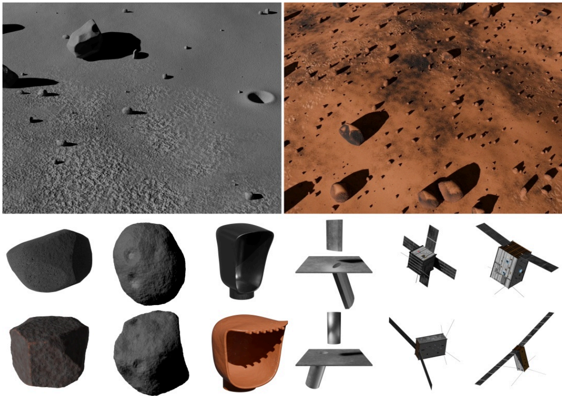
Figure 4.8 – Examples of procedural assets generated by SimForge, including varied terrains, rocks, and structured 3D models like excavation tools, peg-in-hole modules, and spacecraft.
