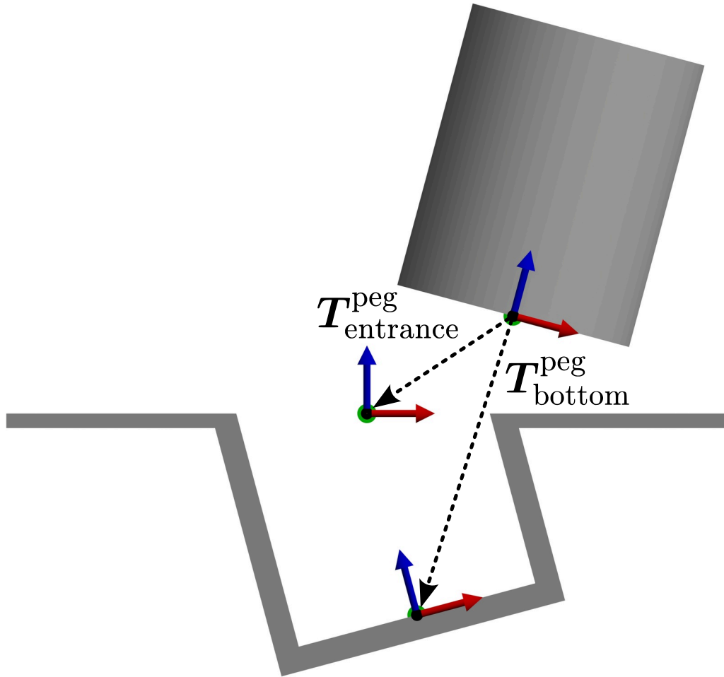
Figure 5.2 – The observation space of the peg-in-hole agents is defined by the T_{entrance}^{peg} and T_{bottom}^{peg} transformations that capture the kinematic state of the assembly.
