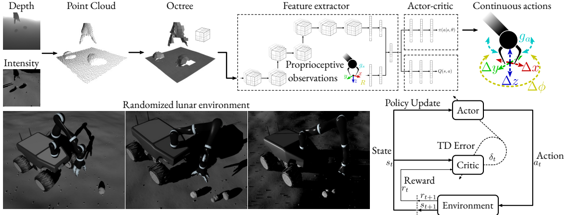
Figure 3.3 – An overview of the end-to-end learning approach. Visual data from a stereo camera is converted into a 3D octree representation. This, along with proprioceptive data, is fed into a shared feature extractor. The resulting features are then used by separate actor and critic networks to produce continuous task-space actions for the robot EE.
