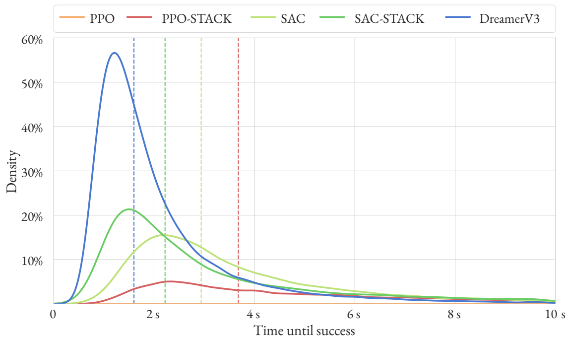
Figure 5.4 – Time until successful completion for the peg-in-hole assembly task. DreamerV3 demonstrates the fastest completion times, followed by the SAC variants.
