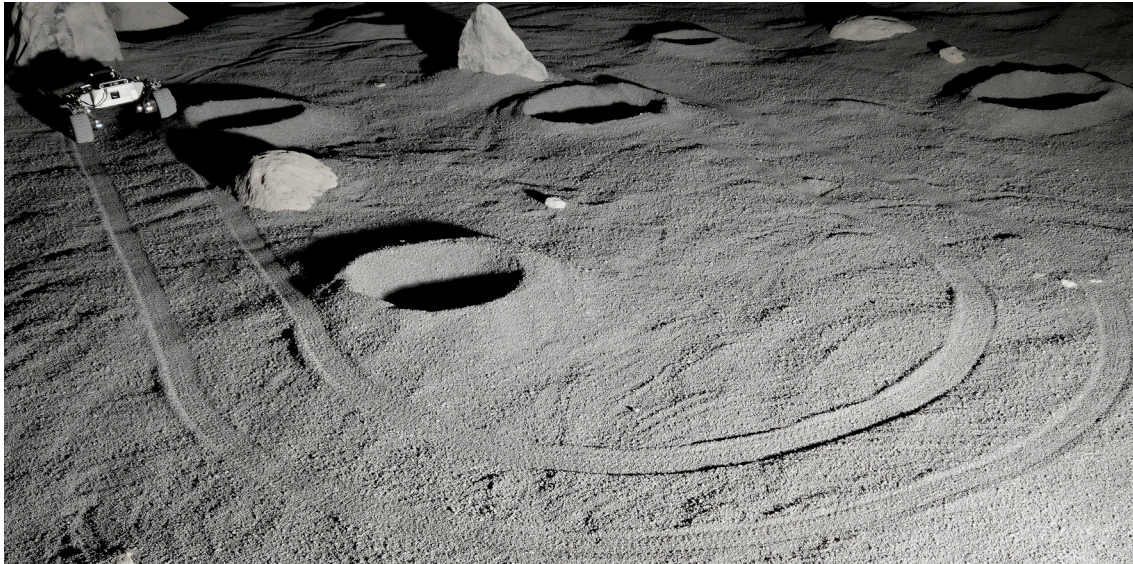
Figure 6.4 – The real-world validation setup in the LunaLab facility with a Leo Rover.
